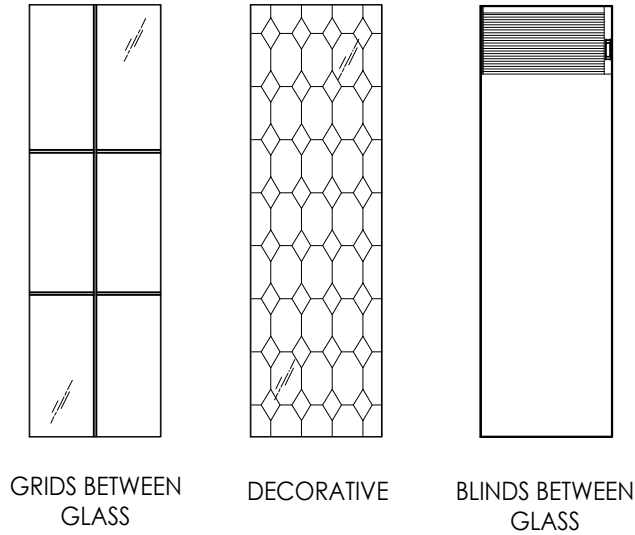
ALTERNATE GLAZING DETAILS
