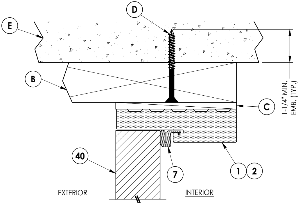
3 4 VERTICAL CROSS SECTION Outswing Shown (Inswing Similar) Shown w/ 2X Buck
