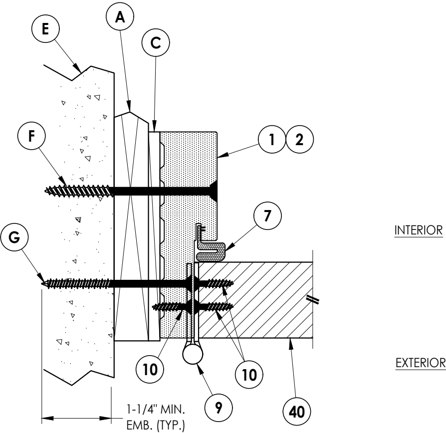
1 HORIZONTAL CROSS SECTION 5 Outswing Shown (Inswing Similar) Shown w/ 1X Buck
