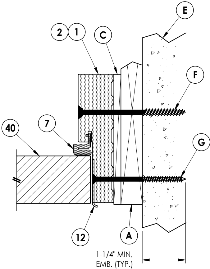
2 HORIZONTAL CROSS SECTION 5 Outswing Shown (Inswing Similar) Shown w/ 1X Buck
