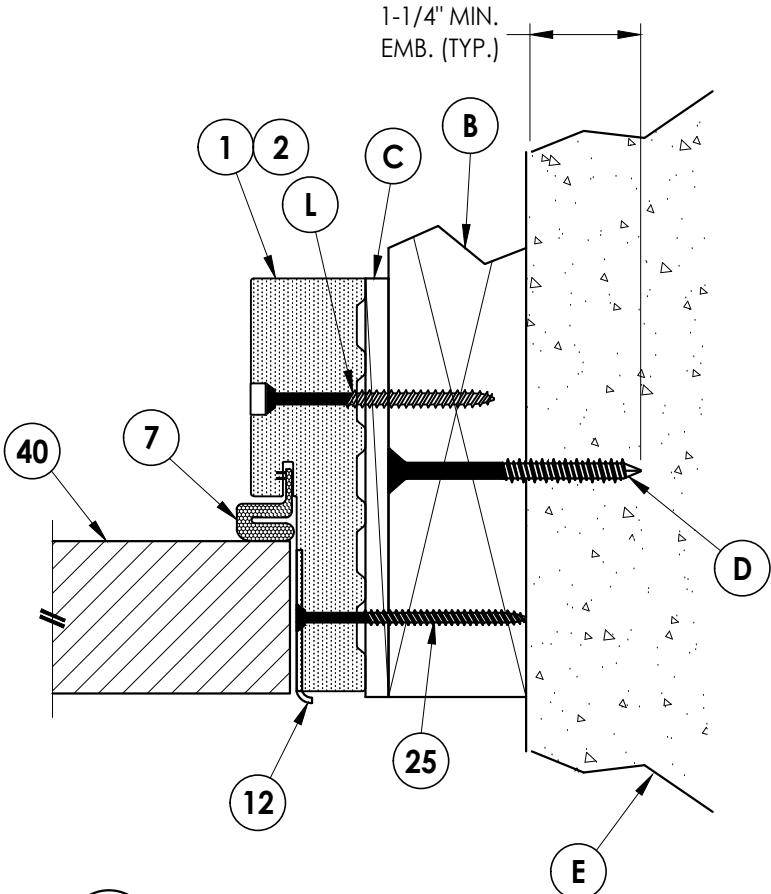
2 4 HORIZONTAL CROSS SECTION Outswing Shown (Inswing Similar) Shown w/ 2X Buck
