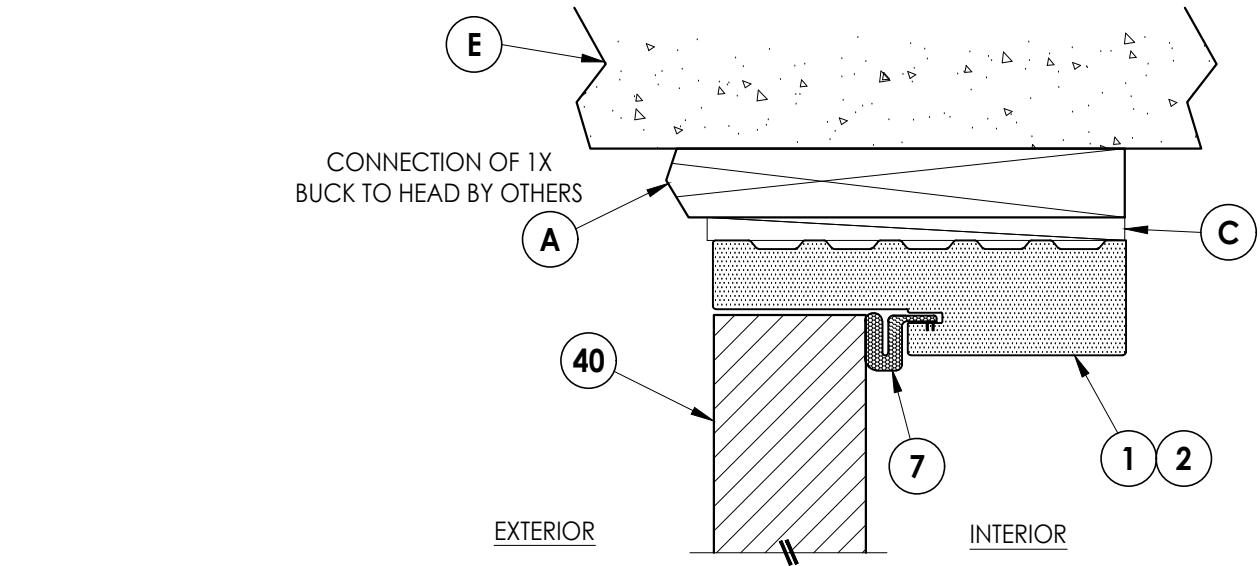
3 VERTICAL CROSS SECTION 5 Outswing Shown (Inswing Similar) Shown w/ 1X Buck
